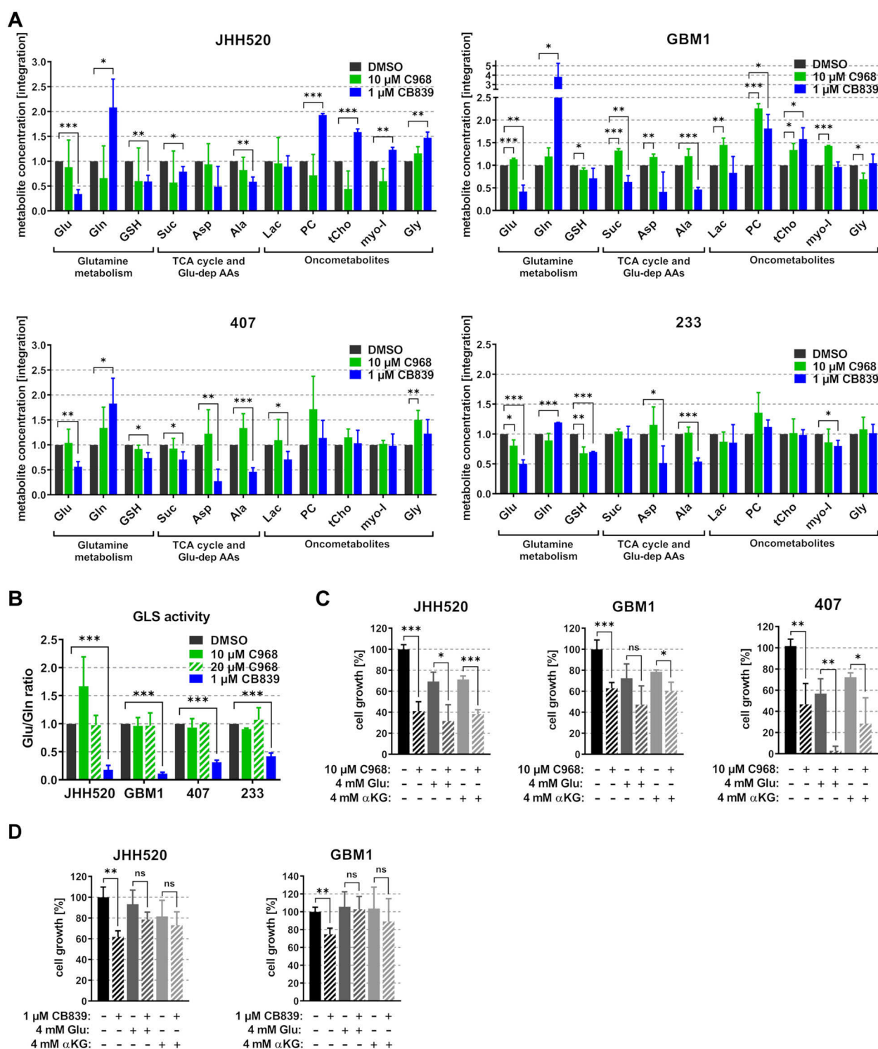
Fig. 5 CB839 effectively blocks glutaminolysis and reduces the influx into the TCA cycle. a Relative metabolite concentrations of GSC cultures treated for 48 h with 10 \mu M C968, 1 \mu M CB839, or DMSO were assessed with HR ^1\text{H} NMR spectroscopy of the water-soluble metabolome ( n = 3 ). b The GLS activity after 48-h treatment with 10 \mu M C968, 20 \mu M C968, 1 \mu M CB839, or DMSO is depicted by the product (Glu) to educt (Gln) ratio of GLS ( n = 3 ). Cell growth of GSCs treated with 10 \mu M C968 ( c ), 1 \mu M CB839 ( d ), or DMSO for 48 h either in the presence of medium only, 4 mM Glu, or 4 mM \alpha KG ( n = 3 ). For all assays, statistical significance was calculated with unpaired t -tests. All data are depicted as mean \pm SD (* p < 0.05 , ** p < 0.01 , *** p < 0.001 ). AA amino acids, \alpha KG alpha ketoglutarate, Ala alanine, Asp aspartate, CFU colony forming units, DMSO dimethylsulfoxid, Gln glutamine, Glu glutamate, Gly glycine, Lac lactate, myo-I myo-inositol, n.s. not significant, PC phosphocholine, ppm parts per million, Suc succinate, TCA tricarboxylic acid, tCho total choline, tCre total creatine.
